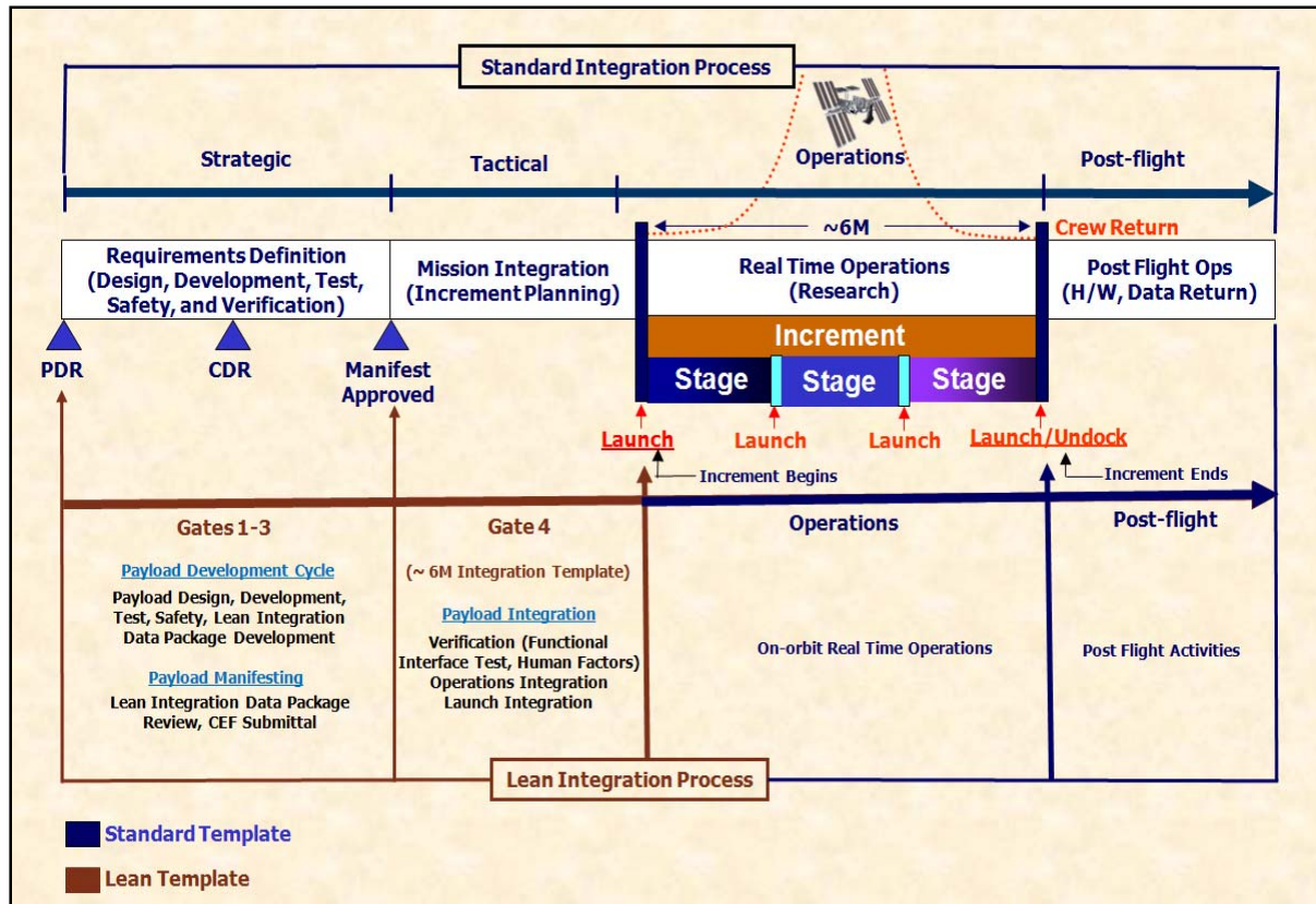
Figure 1 Standard Payload Integration vs. Lean Payload Integration Template
